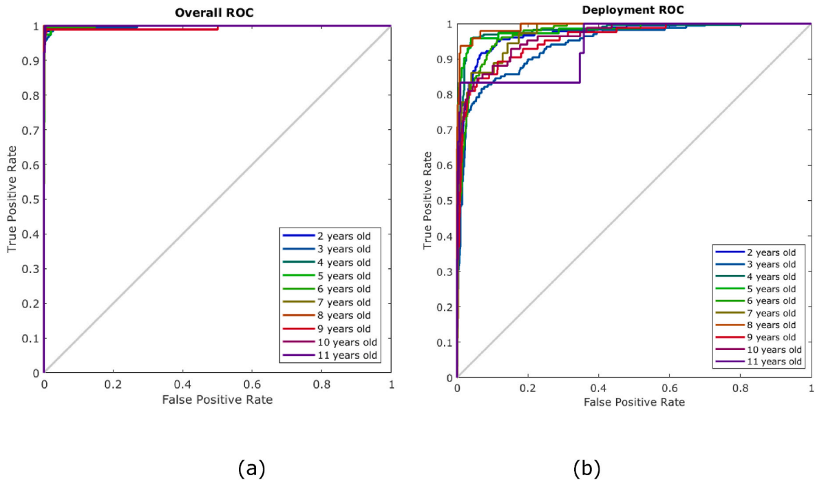
Fig. 7. Receiver operating characteristics (ROC) curves of (a) Model 2 develop with the first data set (N = 1157) and (b) the deployment of Model 2 using the second data set (N = 1068).
