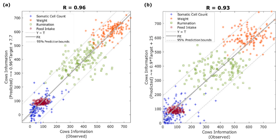
Fig. 6. (a) Regression model (Model 1) developed using data from 150 samples of dairy cows, and (b) deployment of the model using 132 different samples. Abbreviations: R: correlation coefficient; T: targets; cows information refers to the targets/outputs mentioned in the Figure legend.
